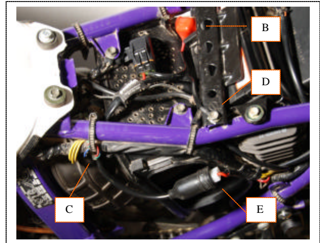
Wiring Harness
